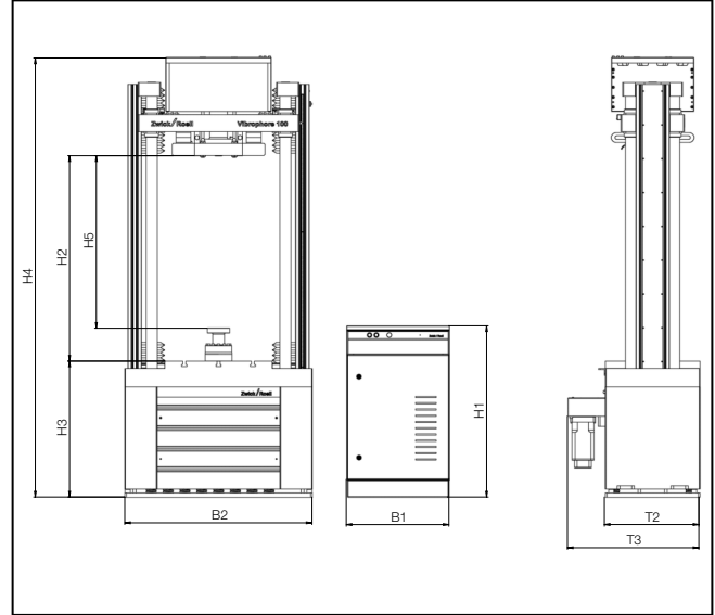
Drawing: Vibrophore 100
